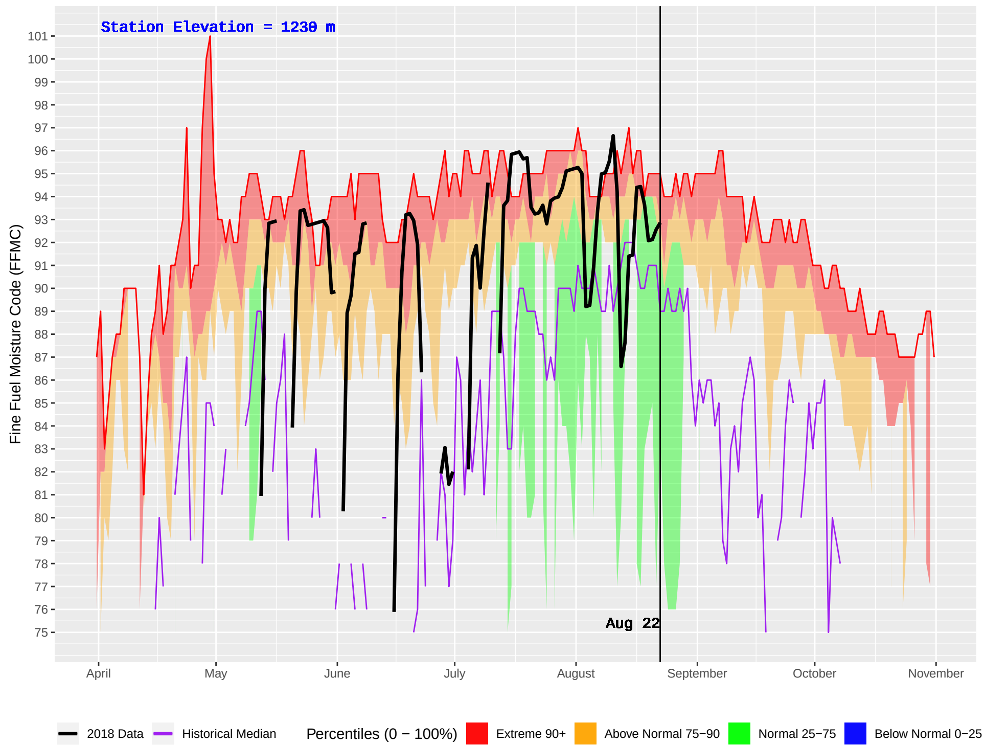
SLOCAN (406) : Historical (1992–2016) and Current (2018) Daily Fine Fuel Moisture Code (FFMC)
