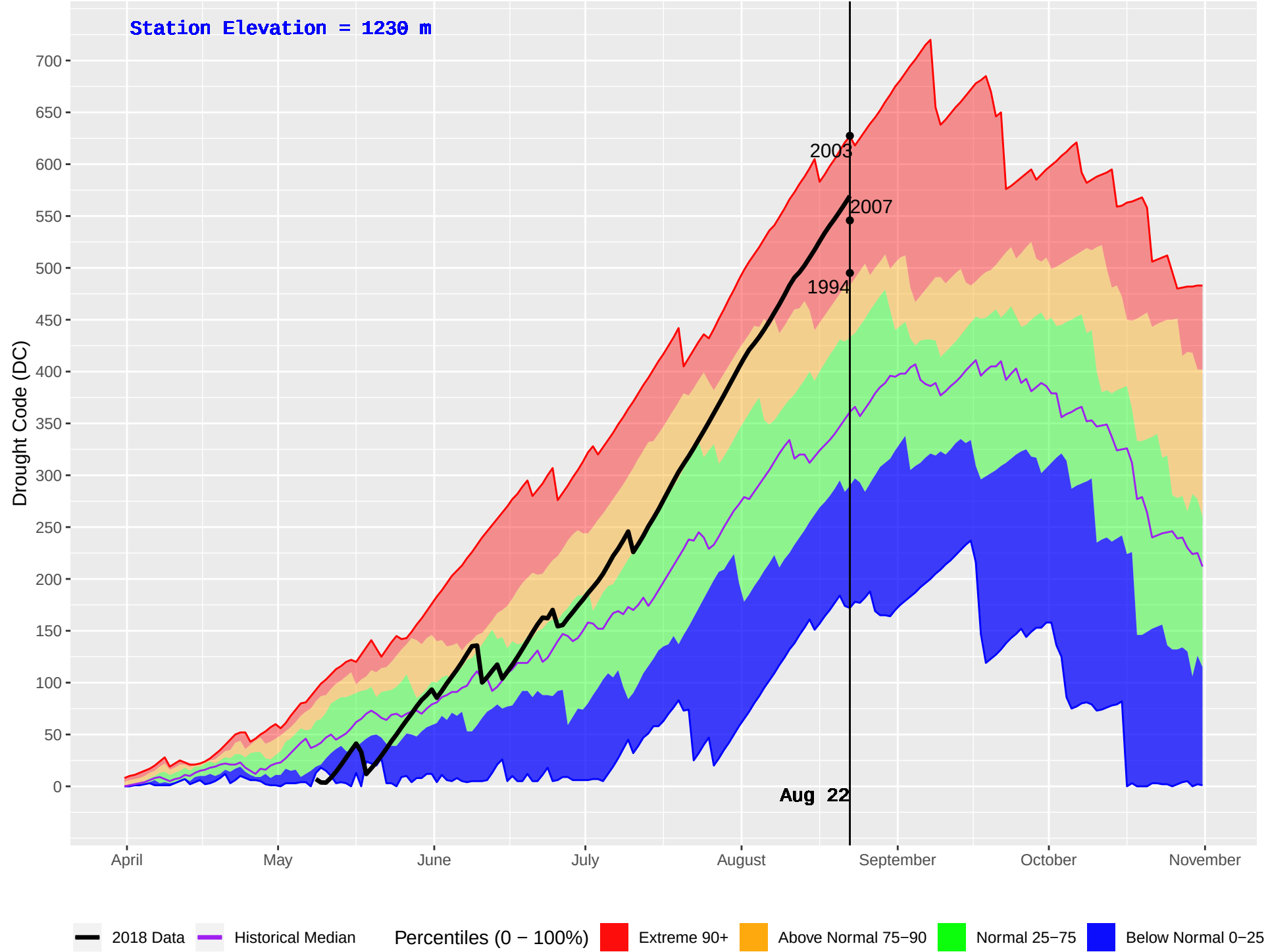
SLOCAN (406) : Historical (1992–2016) and Current (2018) Daily Drought Code (DC)
