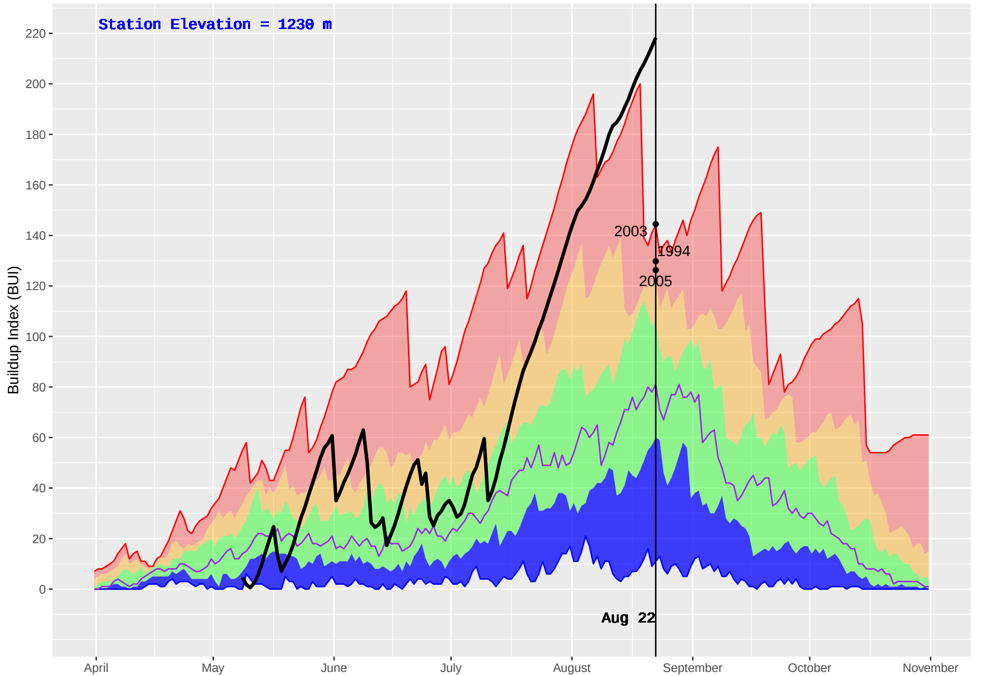
SLOCAN (406) : Historical (1992–2016) and Current (2018) Daily Buildup Index (BUI)
