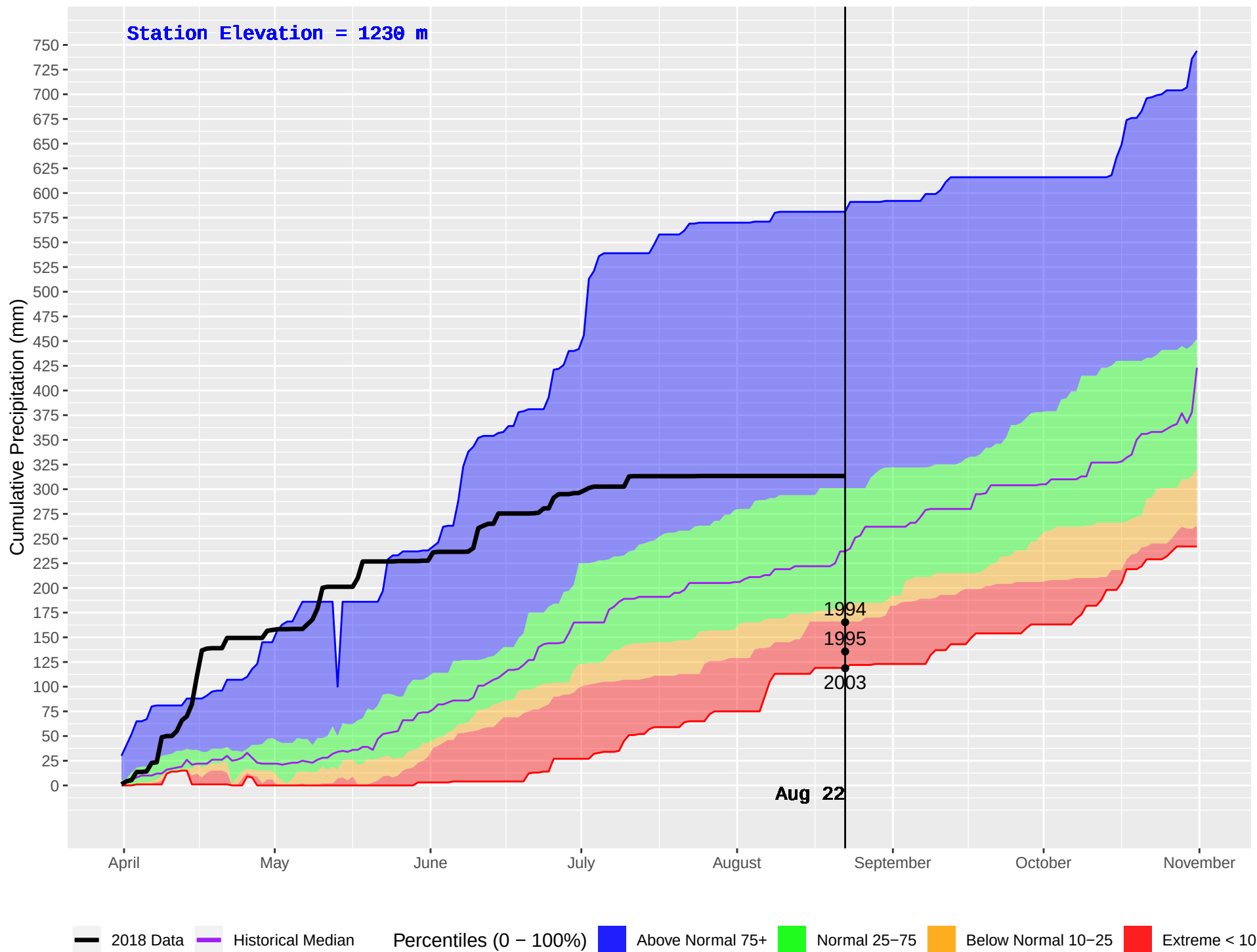
SLOCAN (406) : Historical (1992–2016) and Current (2018) Daily Cumulative Precipitation
