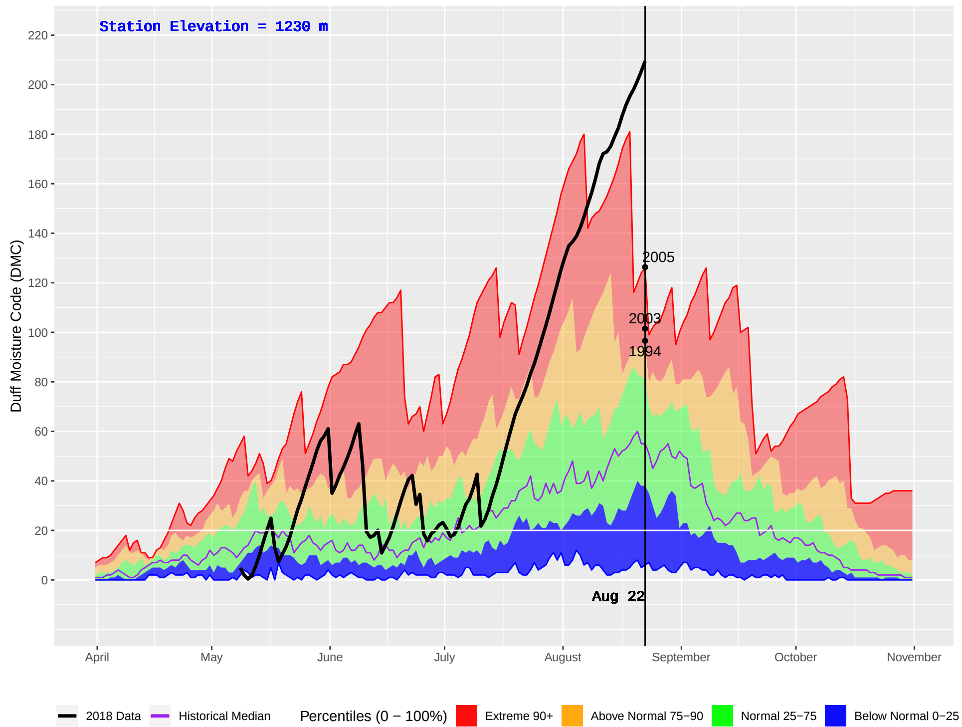
SLOCAN (406) : Historical (1992–2016) and Current (2018) Daily Duff Moisture Code (DMC)
