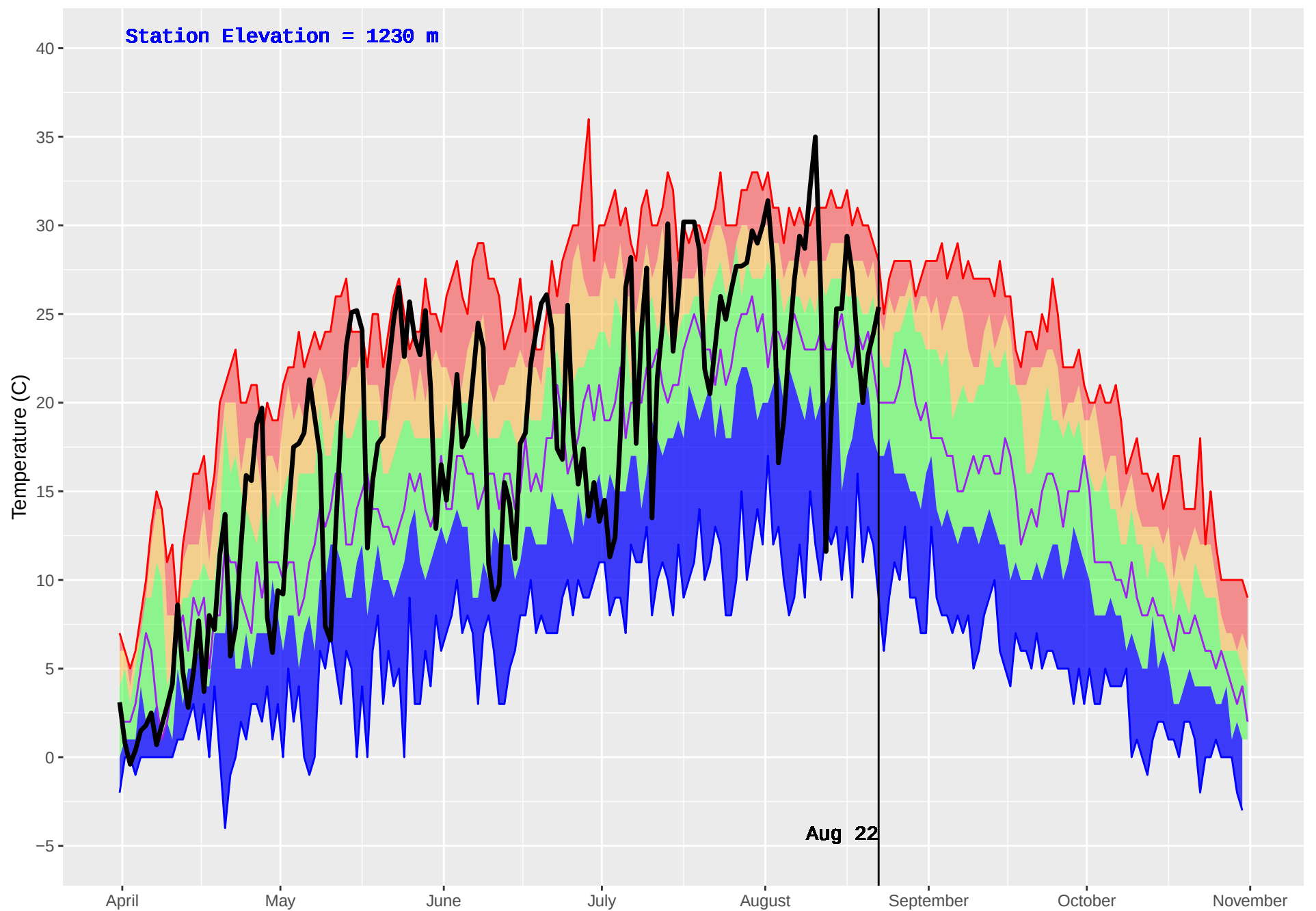
SLOCAN (406) : Historical (1992–2016) and Current (2018) Daily Temperature
