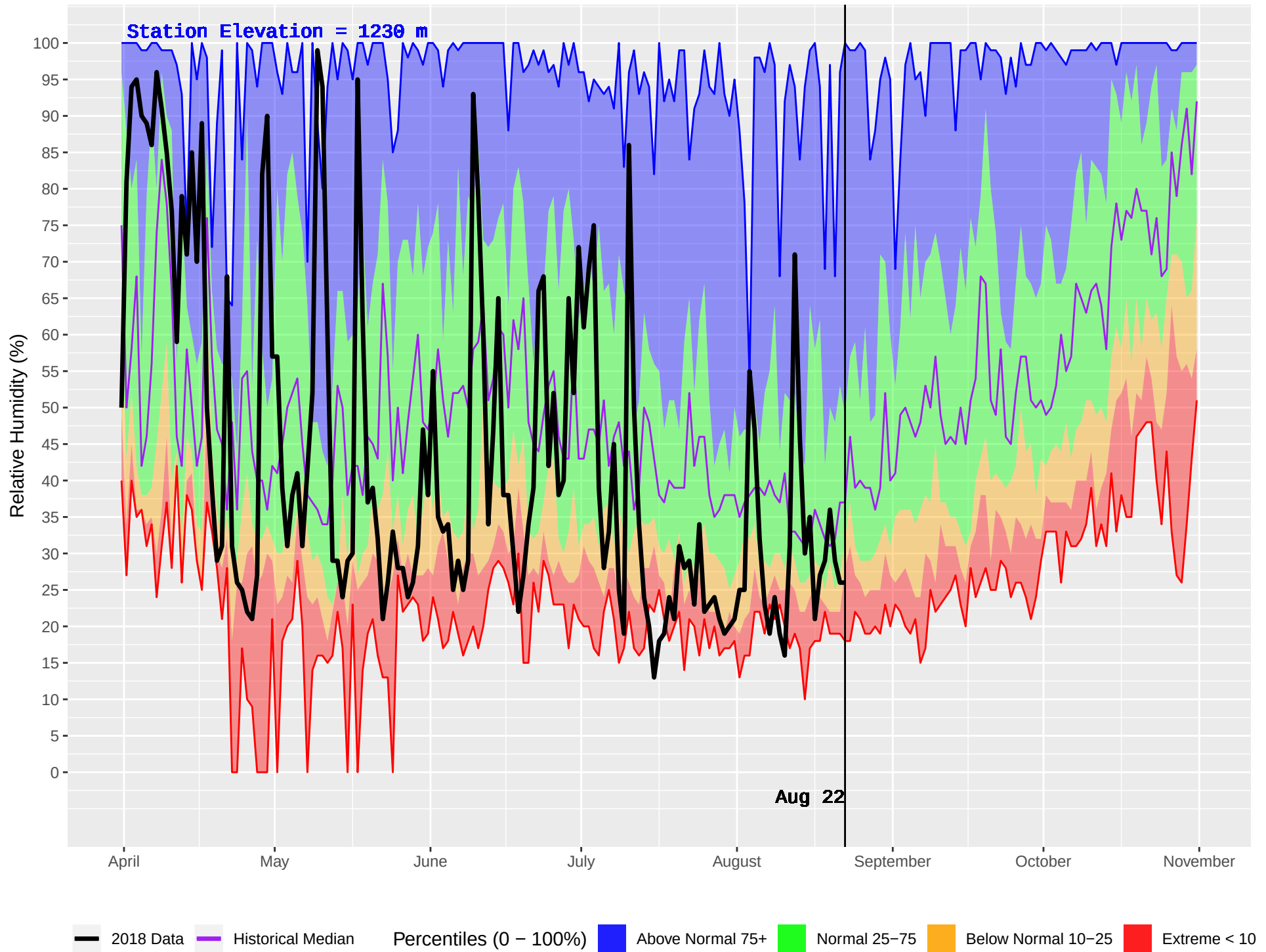
SLOCAN (406) : Historical (1992–2016) and Current (2018) Daily Relative Humidity
