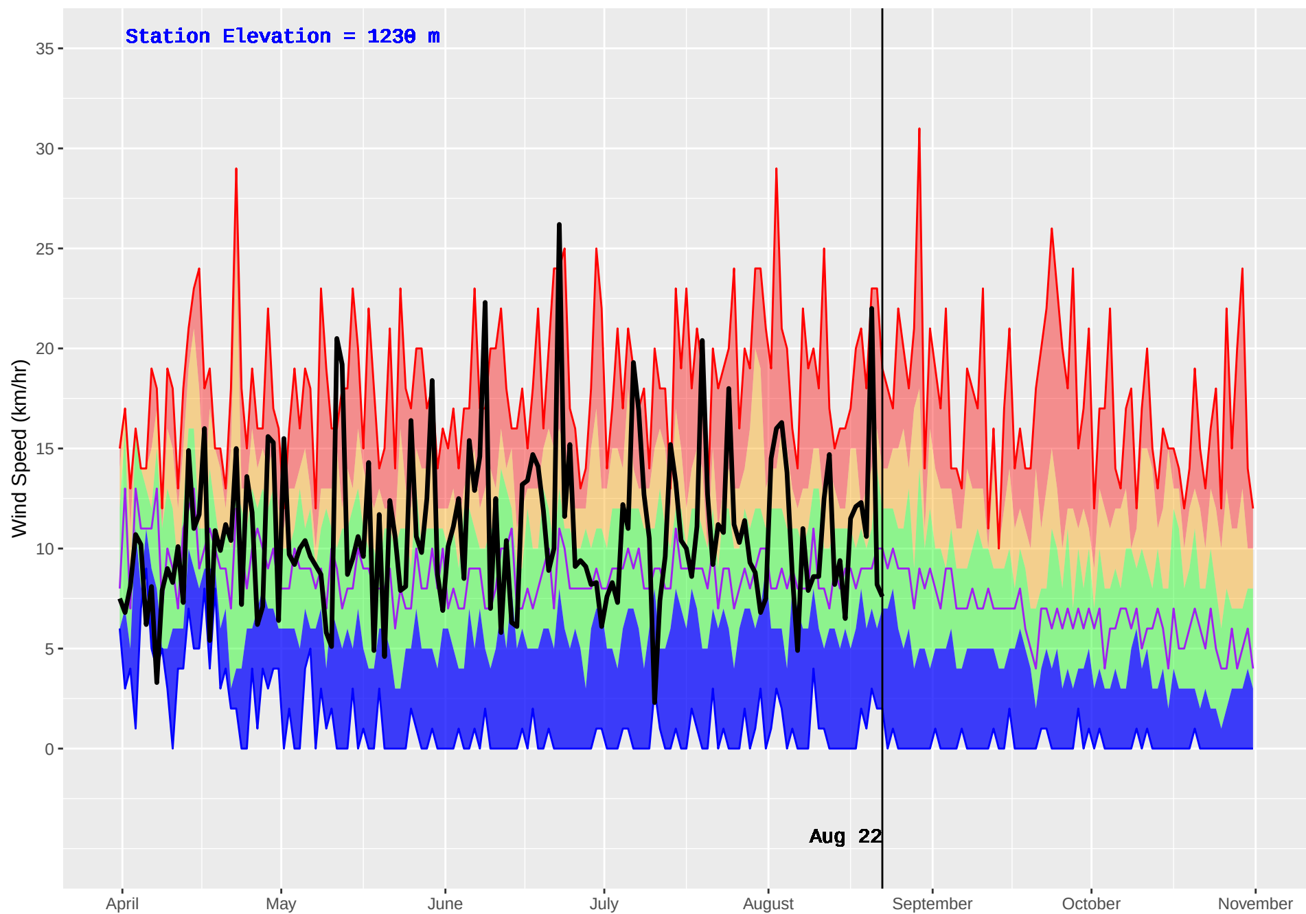
SLOCAN (406) : Historical (1992–2016) and Current (2018) Daily Wind Speed
